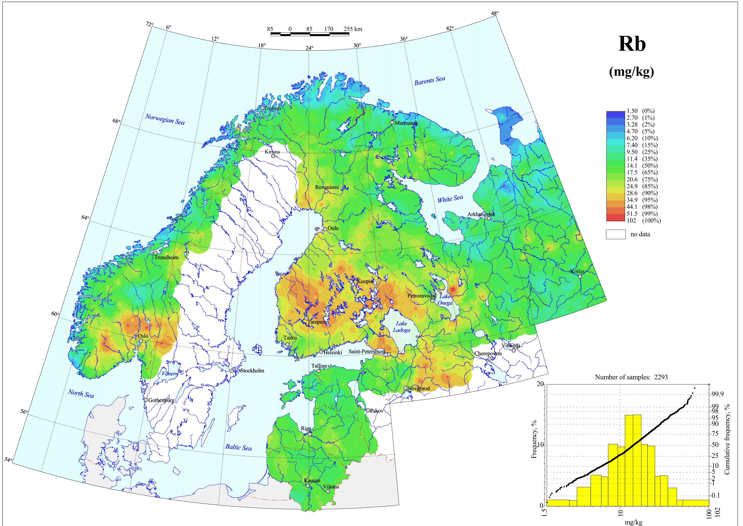
Rubidium in Terrestrial Moss, Total Content
